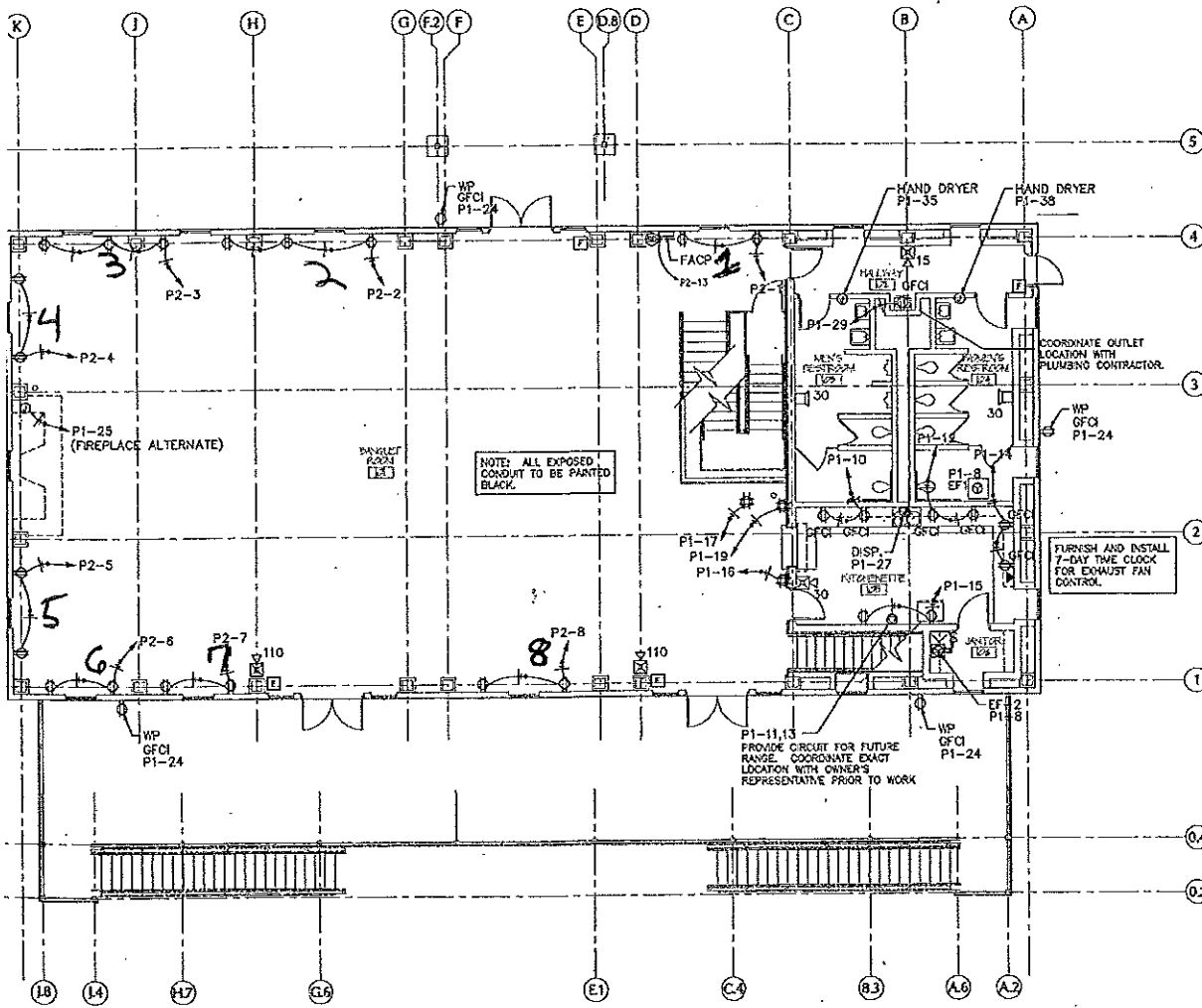
FIRST FLOOR ELECTRICAL POWER PLAN
